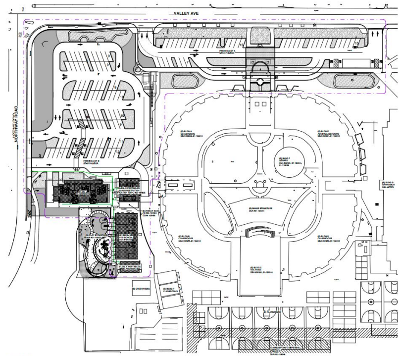
SITE PLAN
