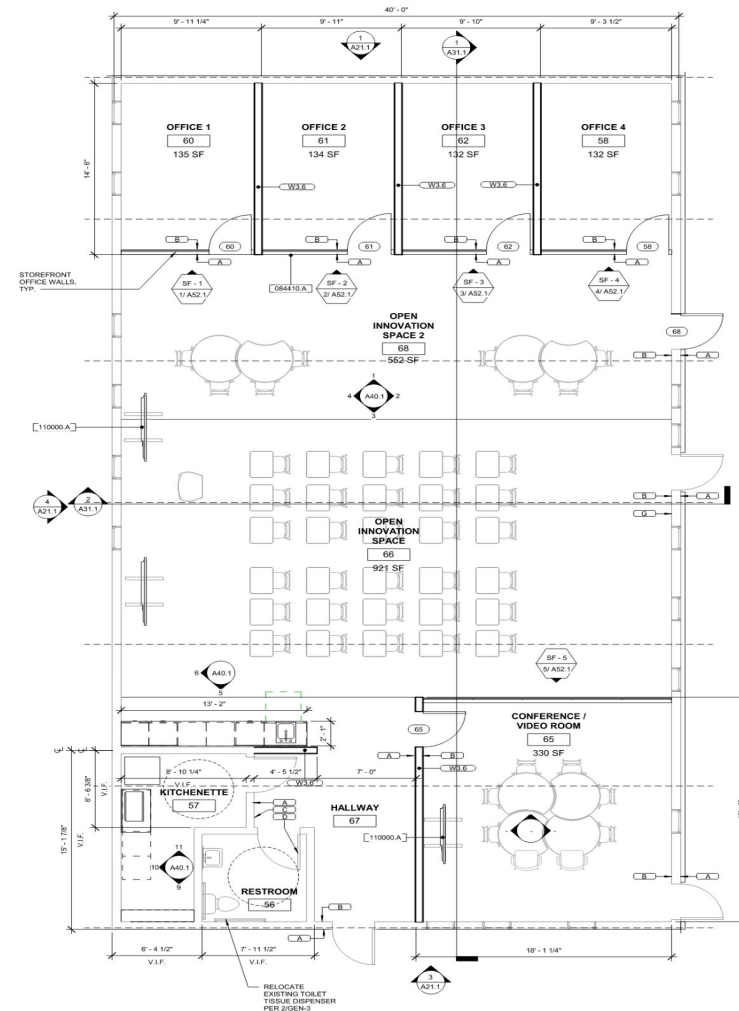
Proposed Layout
