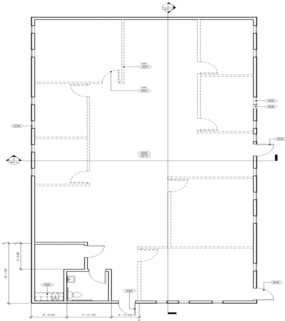
Existing Layout
