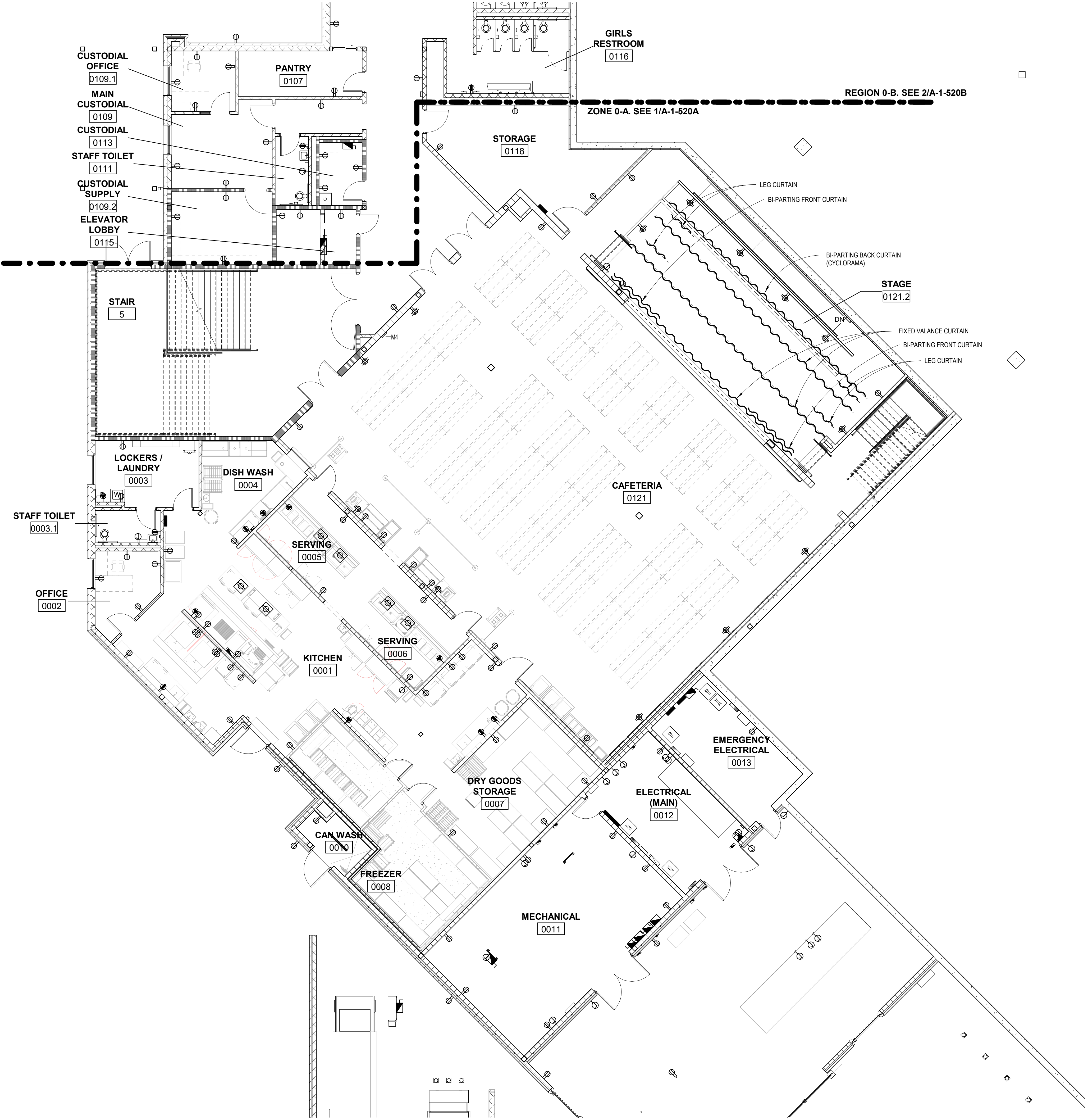
1 FURNITURE PLAN - PHASE 1 - LEVEL 0 - ZONE 0-A 1/8" = 1'-0"
