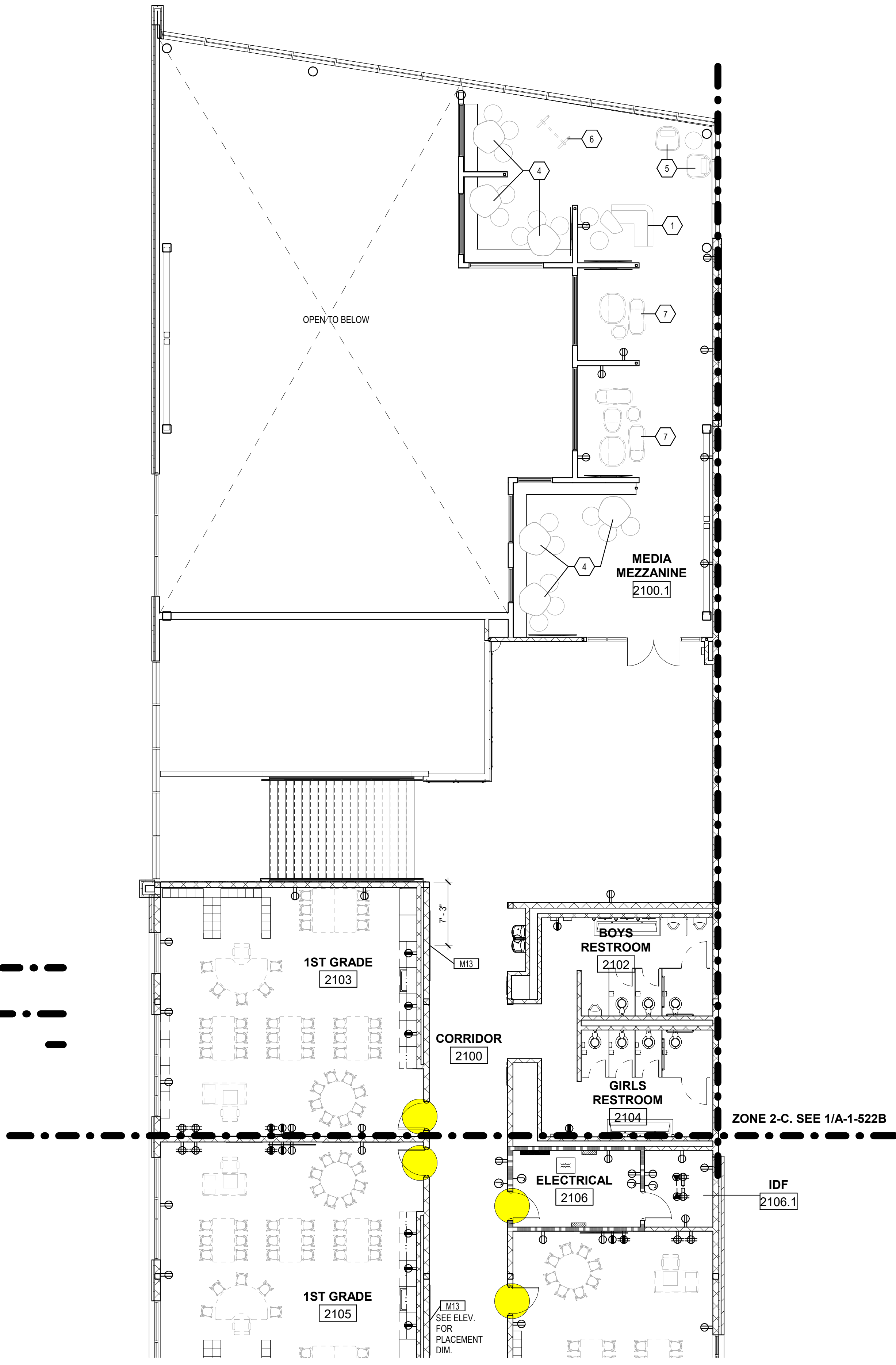
1 FURNITURE PLAN - PHASE 1 - LEVEL 2 - ZONE 2-C 1/8" = 1'-0"
