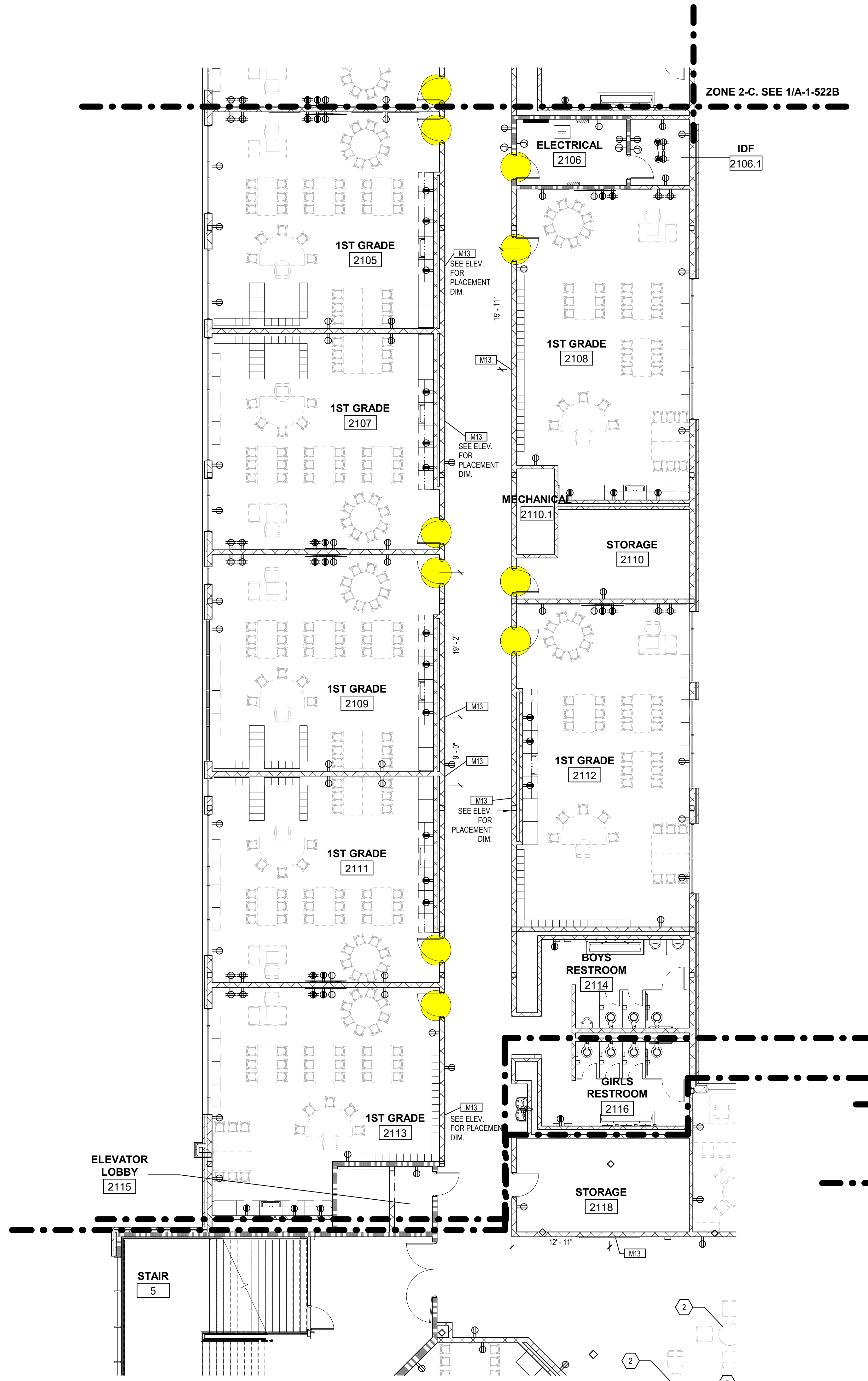
2 FURNITURE PLAN - PHASE 1 - LEVEL 2 - ZONE 2-B 1/8" = 1'-0"
