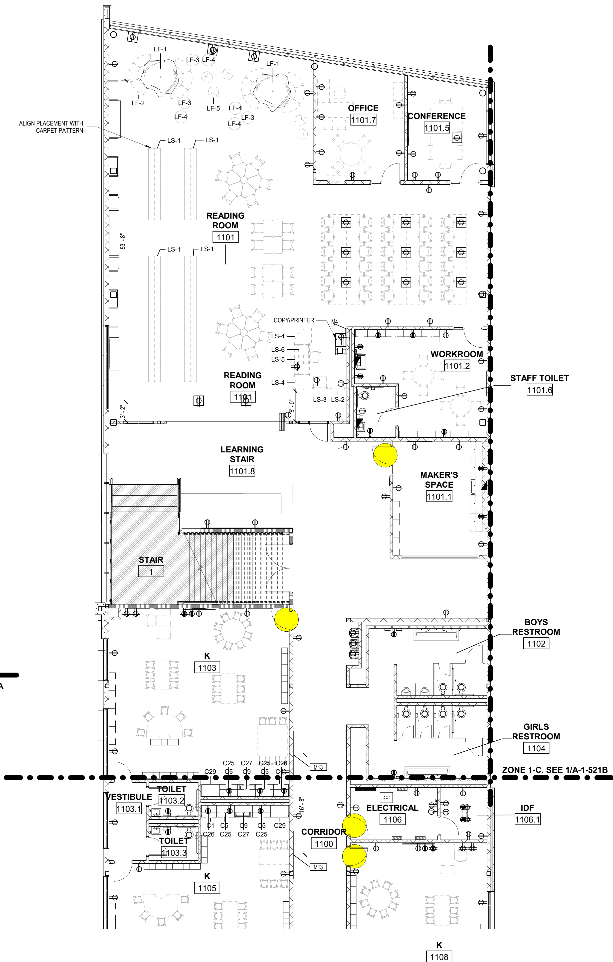
1 FURNITURE PLAN - PHASE 1 - LEVEL 1 - ZONE 1-C 1/8" = 1'-0"
