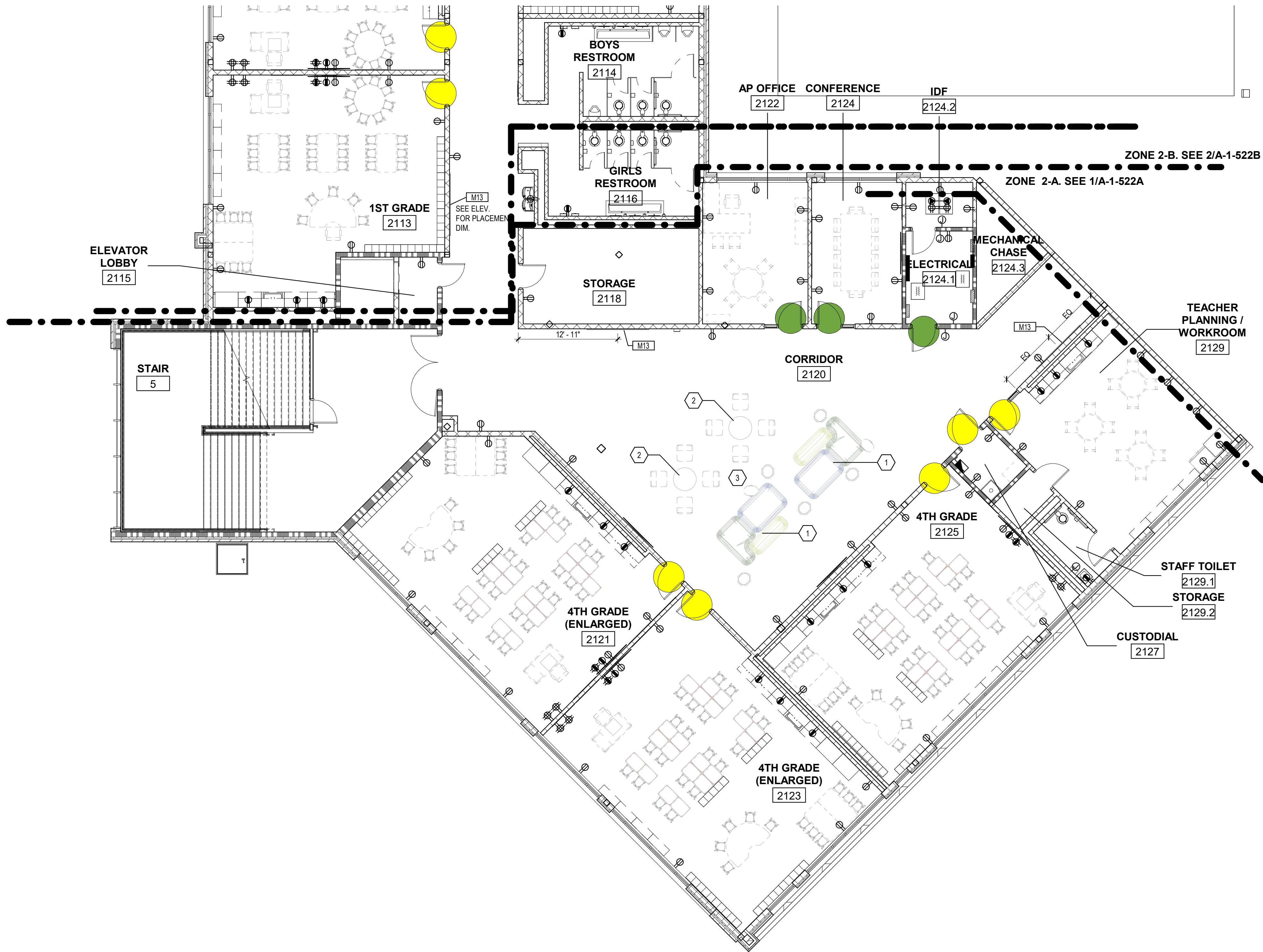
1 FURNITURE PLAN - PHASE 1 - LEVEL 2 - ZONE 2-A 1/8" = 1'-0"
