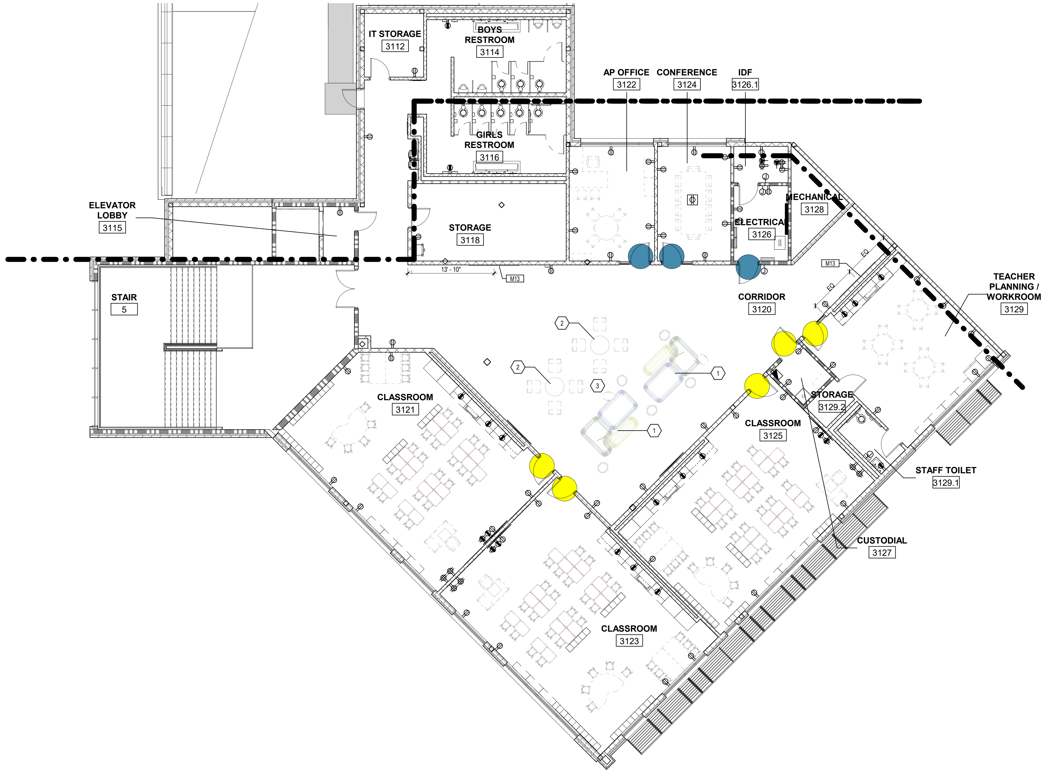
1 FURNITURE PLAN - PHASE 1 - LEVEL 3 - ZONE 3-A 1/8" = 1'-0"
