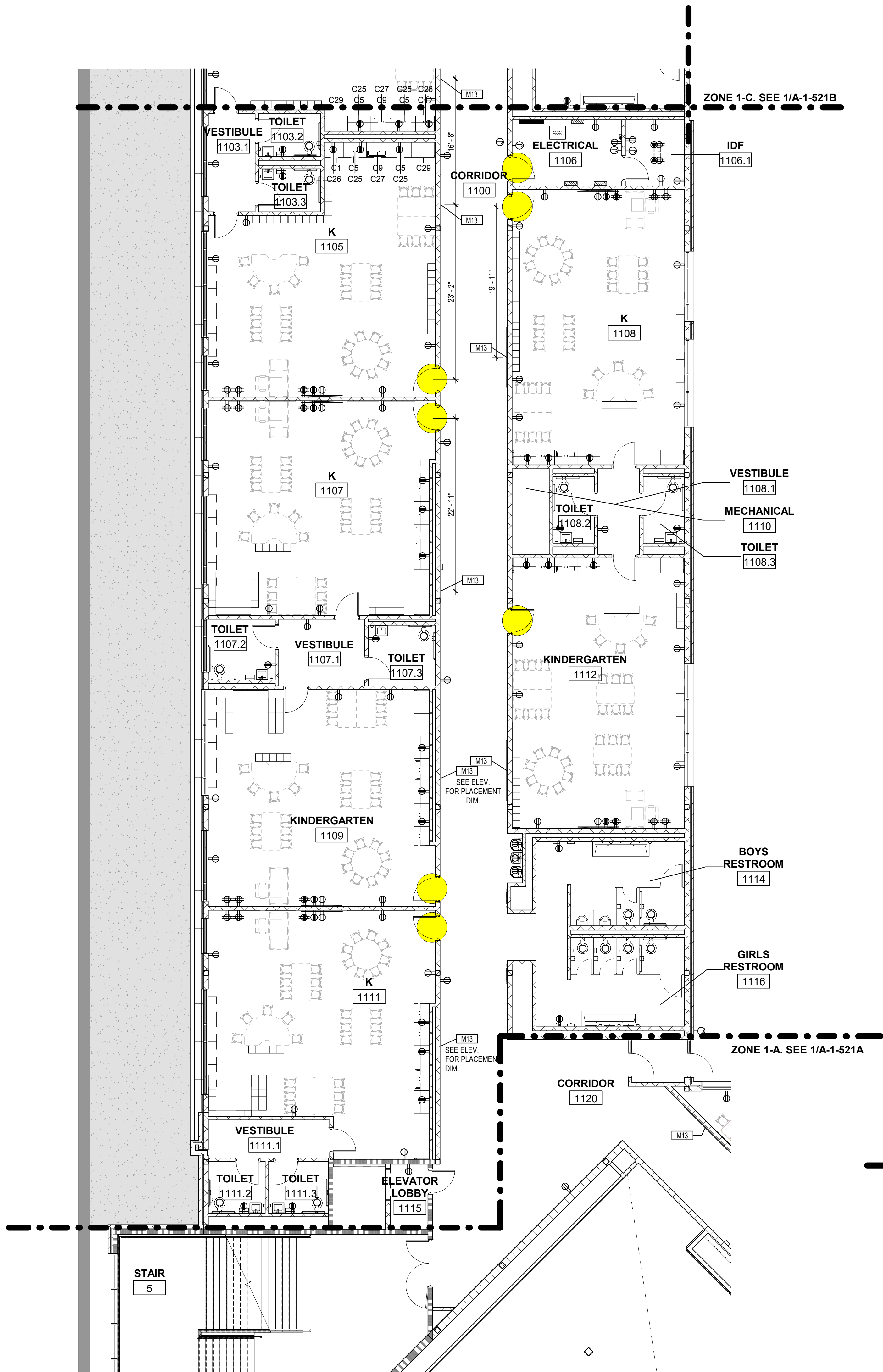
2 FURNITURE PLAN - PHASE 1 - LEVEL 1 - ZONE 1-B 1/8" = 1'-0"
