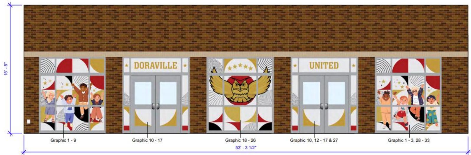
① Elevation 1 1/4" = 1'-0"
