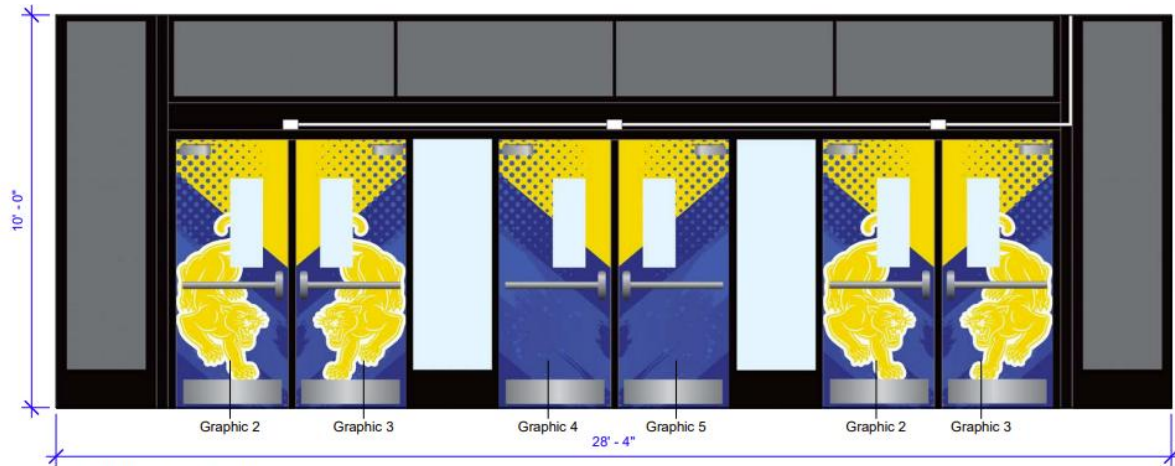
① Elevation 1 - Entry 1 3/8" = 1'-0"
