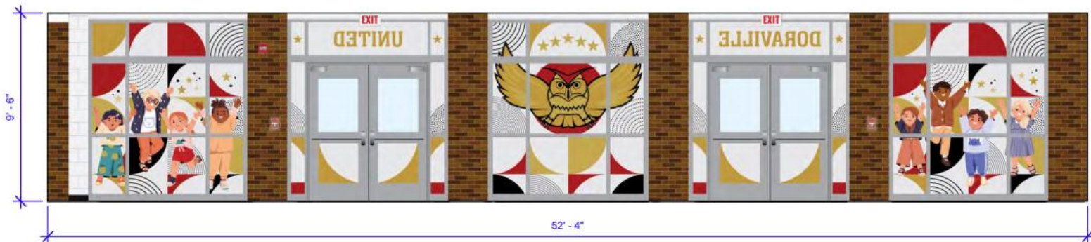
① Elevation 1 1/4" = 1'-0"
