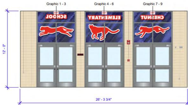
③ Elevation 3 1/4" = 1'-0"
