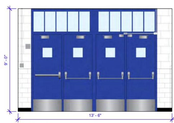
⑦ Elevation 7 3/8" = 1'-0"
