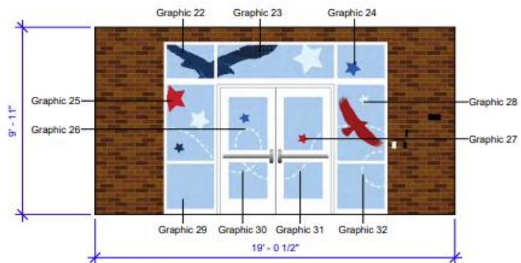
⑤ Elevation 5 1/4" = 1'-0"
