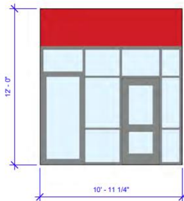
④ Elevation 4 1/4" = 1'-0"
