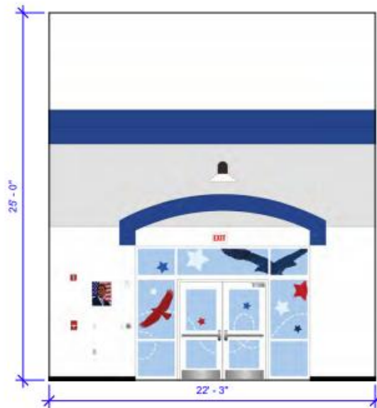
② Elevation 2 3/16" = 1'-0"
