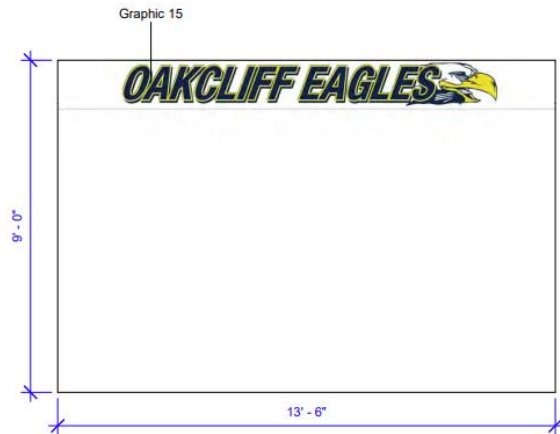
⑧ Elevation 8 3/8" = 1'-0"
