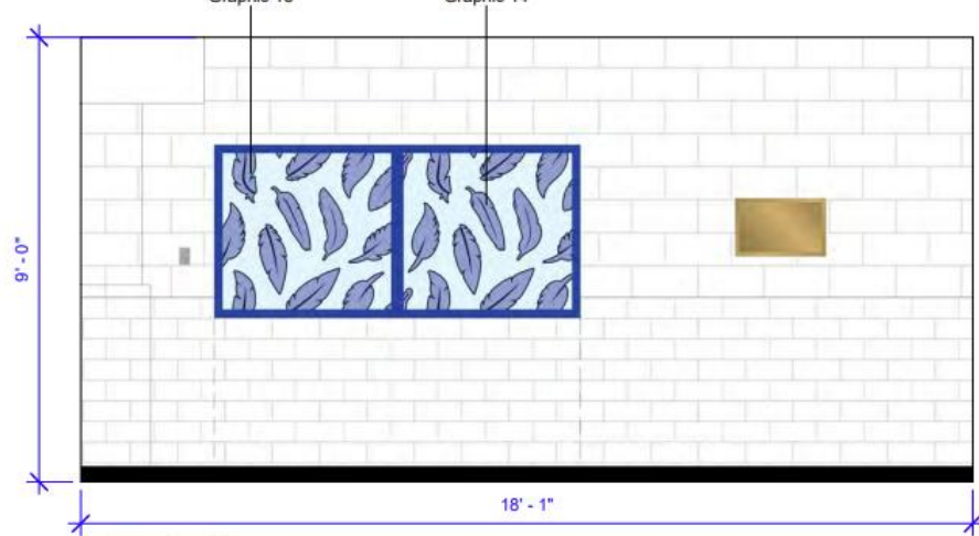
⑥ Elevation 6 3/8" = 1'-0"
