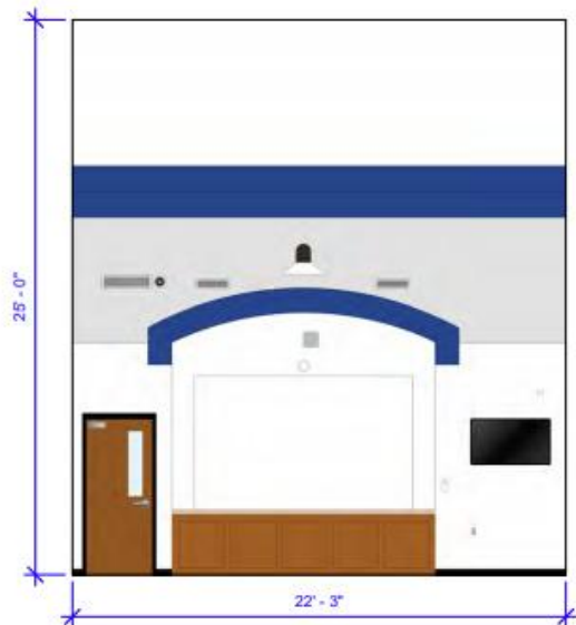
④ Elevation 4 3/16" = 1'-0"
